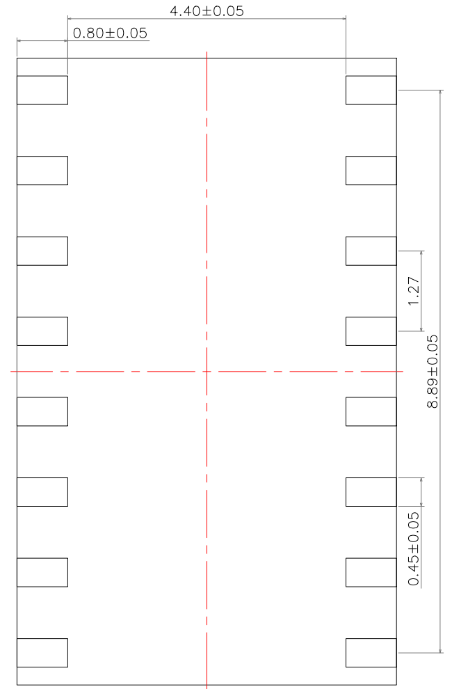
BOTTOM VIEW
