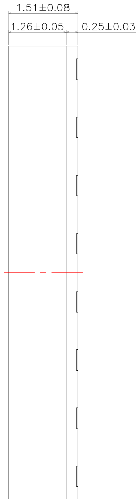
SIDE VIEW
